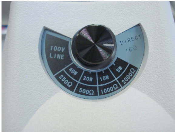
Fig.3. B5/T & B6/T power selector
