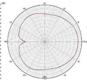
Fig. 6. Cardioid pattern
